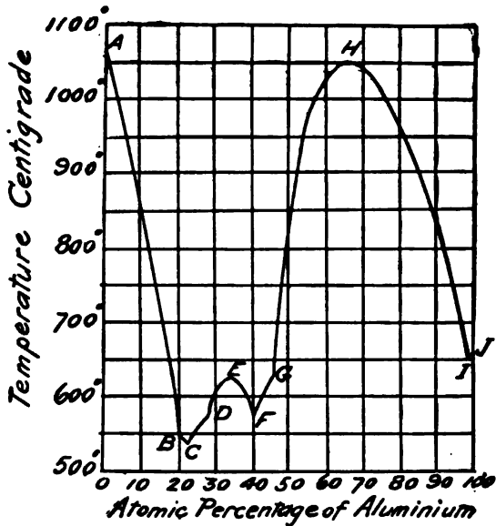
Fig. 52. Freezing-point Curve of the Gold-aluminium Alloys.
